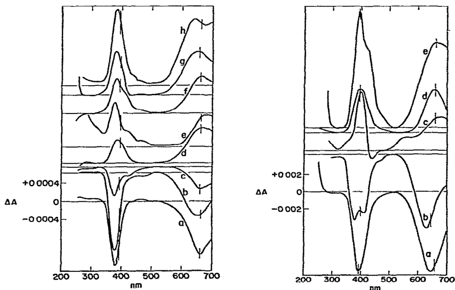
Fig. 2 CD spectra of low-pH complexes of \text{Ni}^{\text{II}} with hydroxy acids. \text{Ni}^{\text{II}} about 0.16 normal, 10-mm cell. Dichroism in absorbancy units, scale indicated. Vertical bars, location of maxima of absorption bands (a) Lactic acid, 5:1, pH 7; (b) arabonic acid, 3:1, pH 7; (c) arabonic acid, 1:1.1, pH 6; (d) gluconic acid, 2:1, pH 4; (e) galactonic acid, 3:1, pH 6; (f) xylonic acid, 1:5.1, pH 6; (g) gulonic acid, 5:1, pH 3; (h) ribonic acid, 3:1, pH 6.
