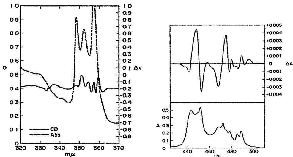
Fig. 10. Absorption and CD spectra of \text{Nd}^{\text{III}} in alkaline tartrate, 320–370-nm region.
