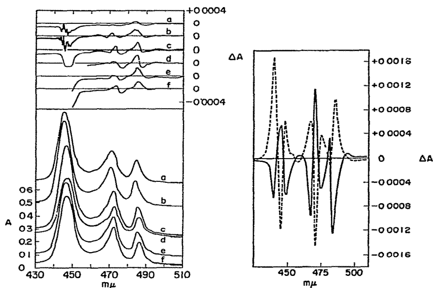
Fig 8 CD and absorption spectra for aspartic acid-Pr III mixtures, with increasing pH, (a) 2 l, pH 6, (b)-(d), 3:1, pH 6, 8, 9, respectively; (e), (f), 5 l, pH 8, 9, respectively. CD pathlengths, 30 mm, absorption, 5 mm
